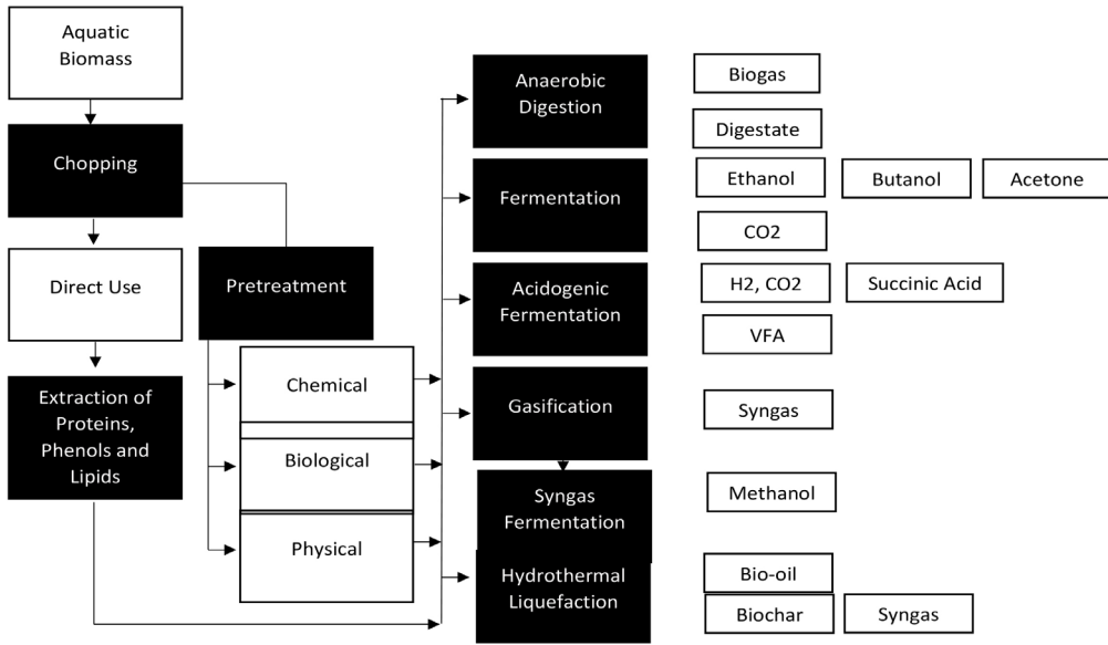
Figure 1: Main processing strategies in aquatic biorefineries
